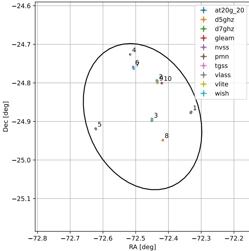
4FGL J1910.0-2453
