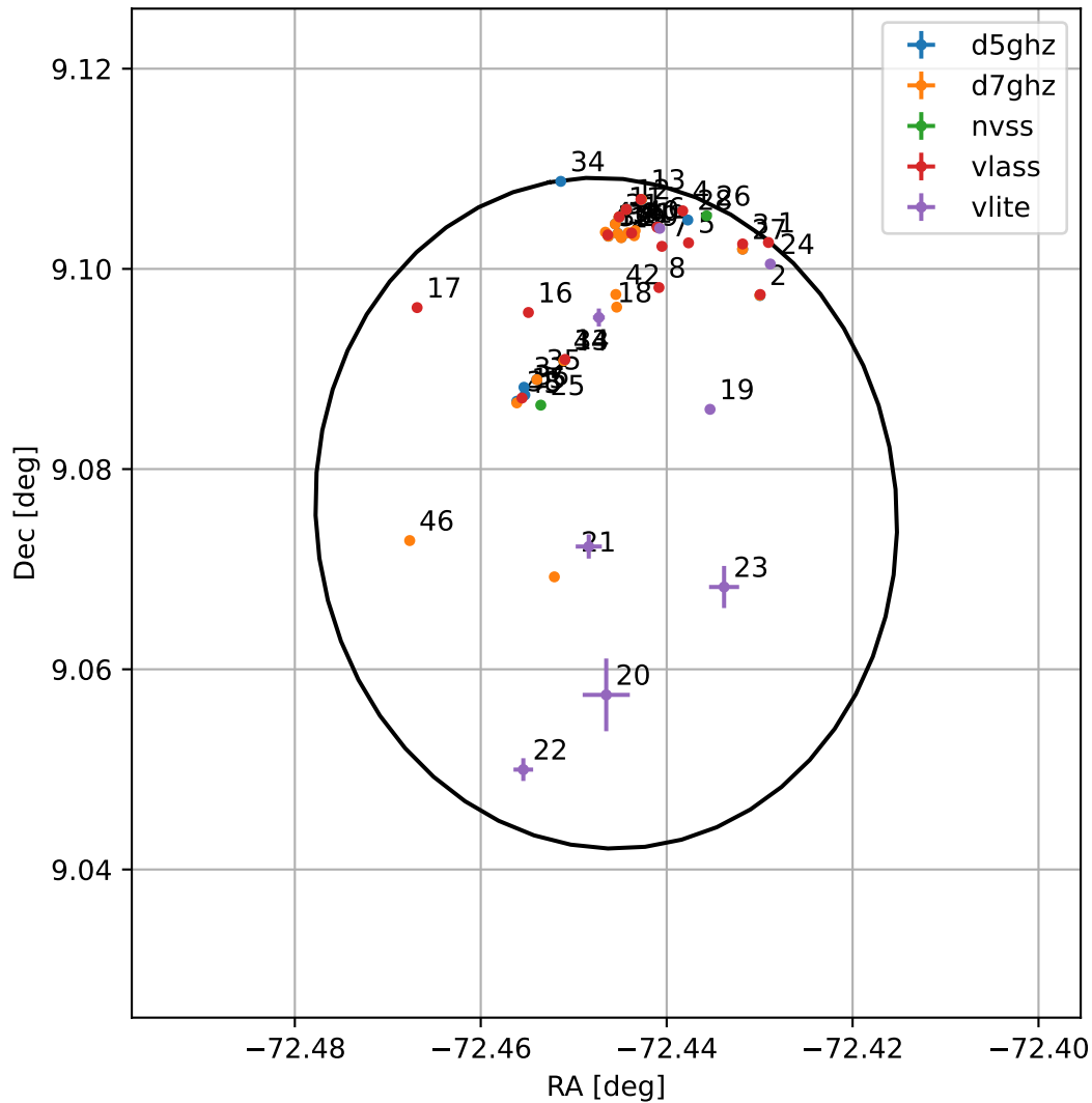
4FGL J1910.2+0904
