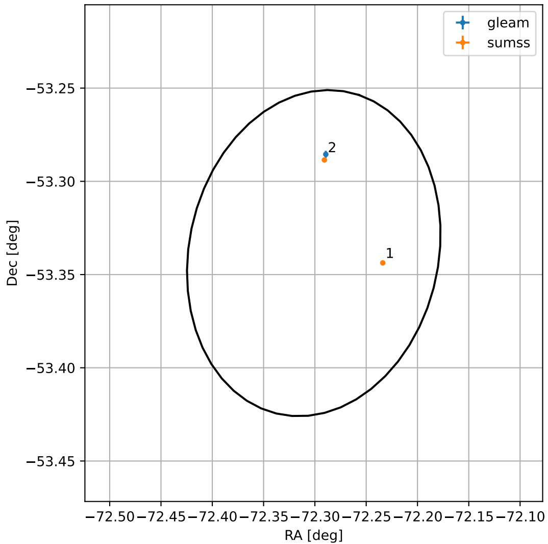
4FGL J1910.7-5320
