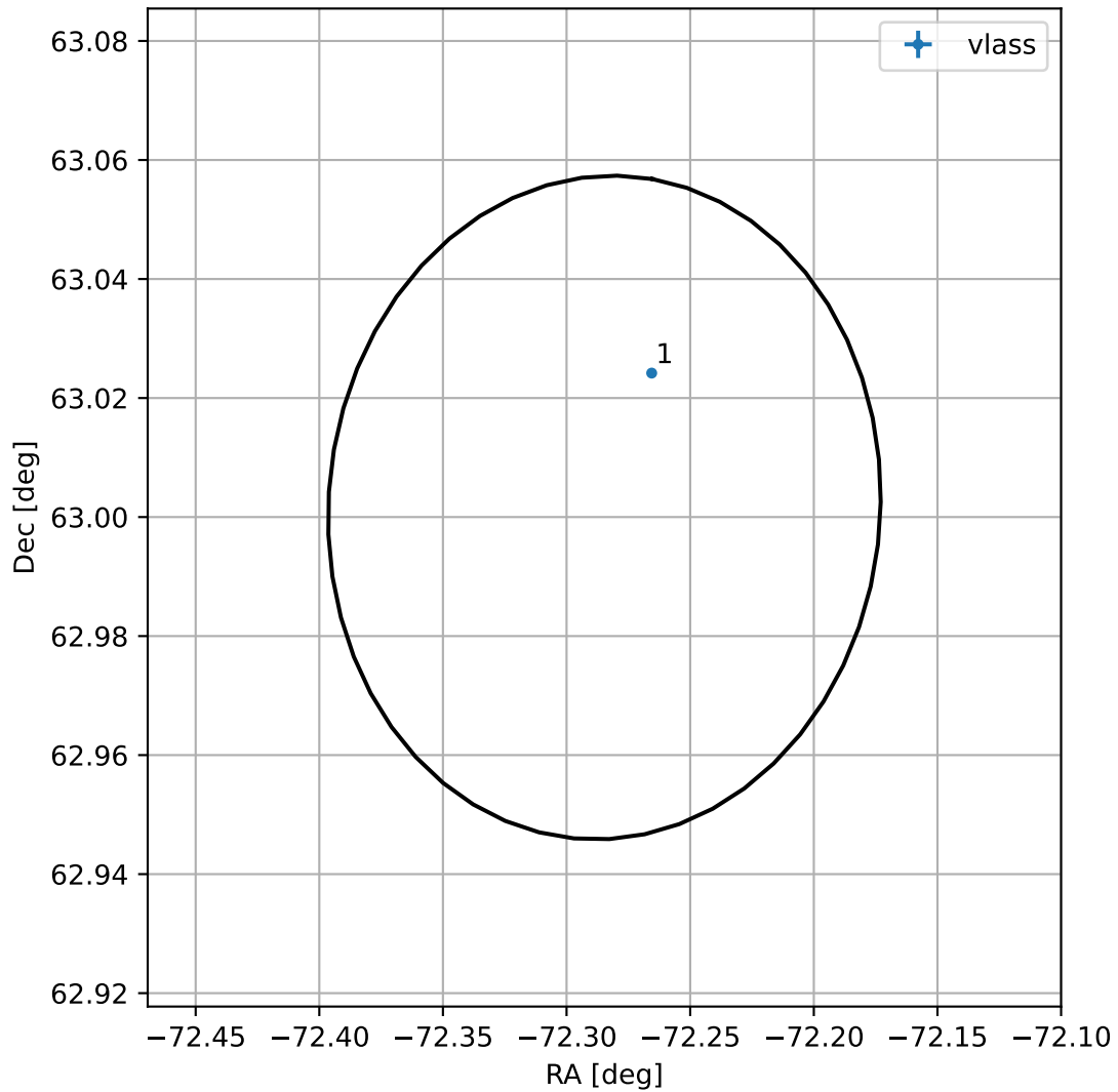
4FGL J1910.8+6300
