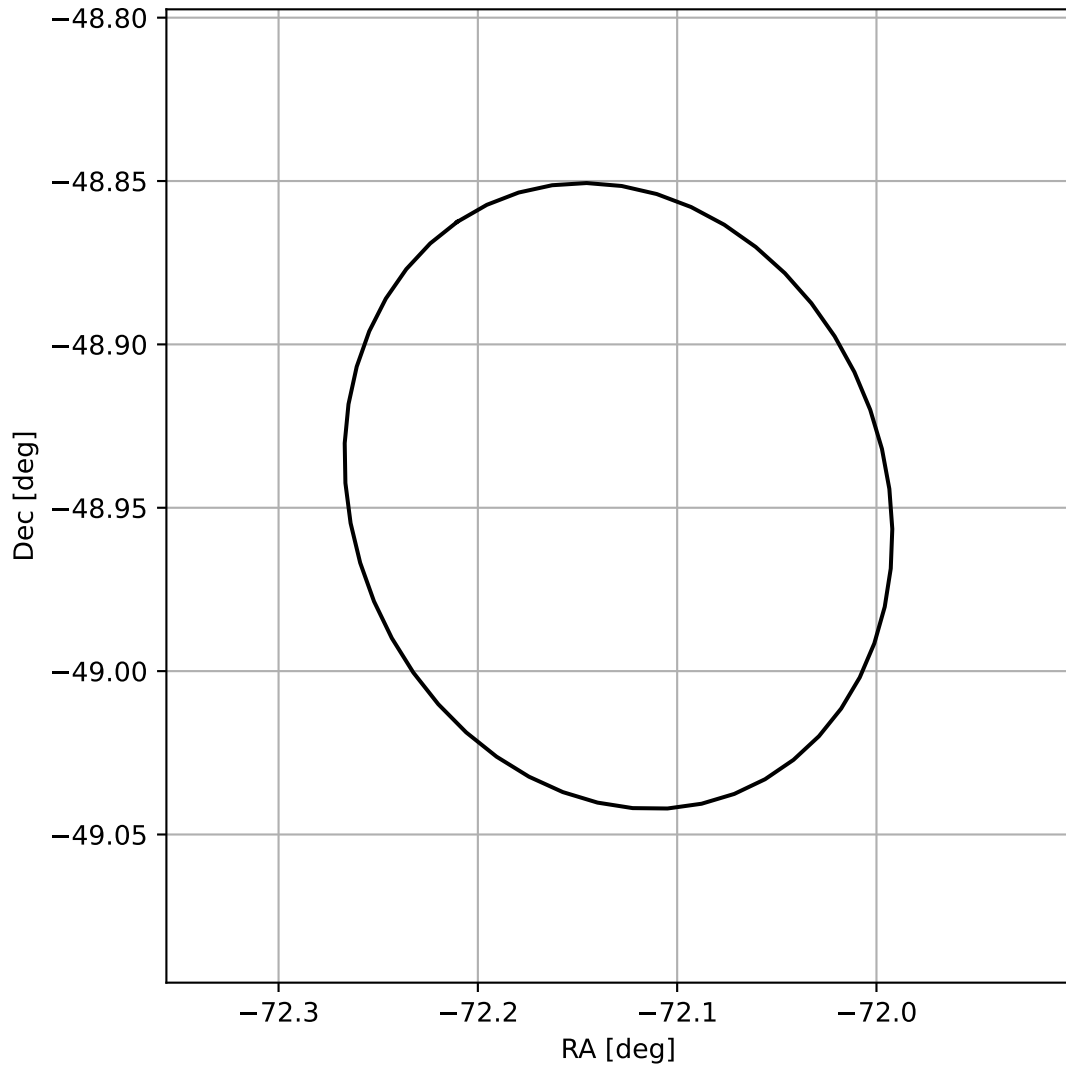
4FGL J1911.4-4856
