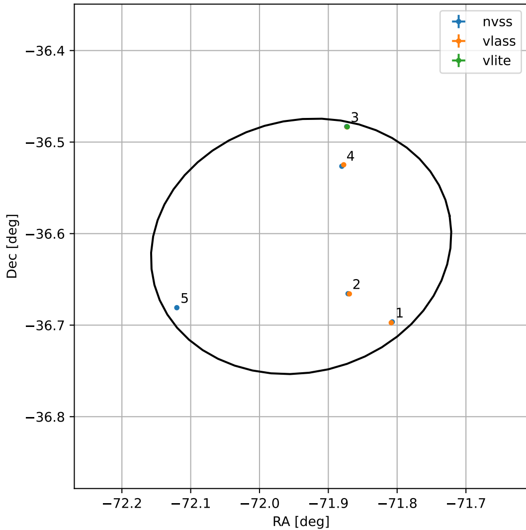
4FGL J1912.2-3636
