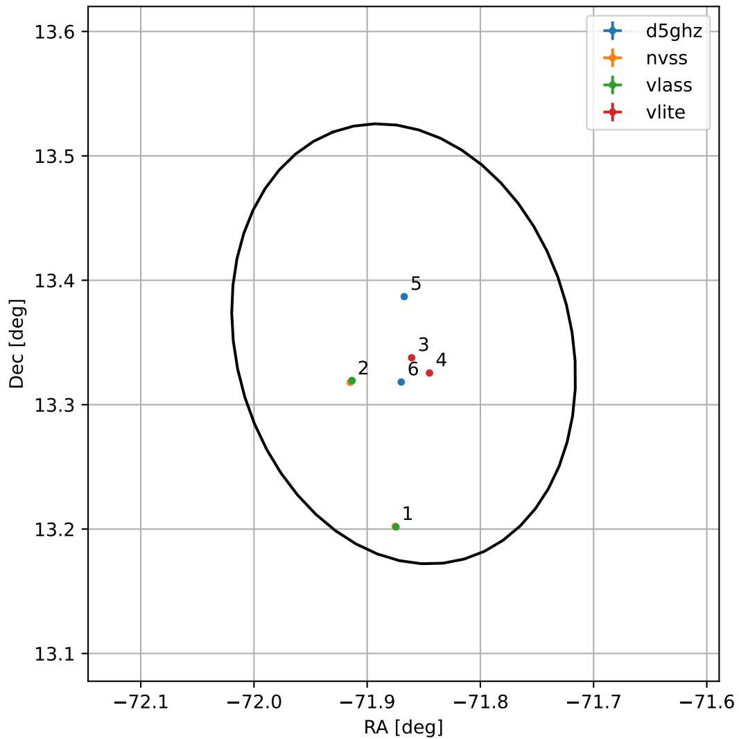
4FGL J1912.5+1320
