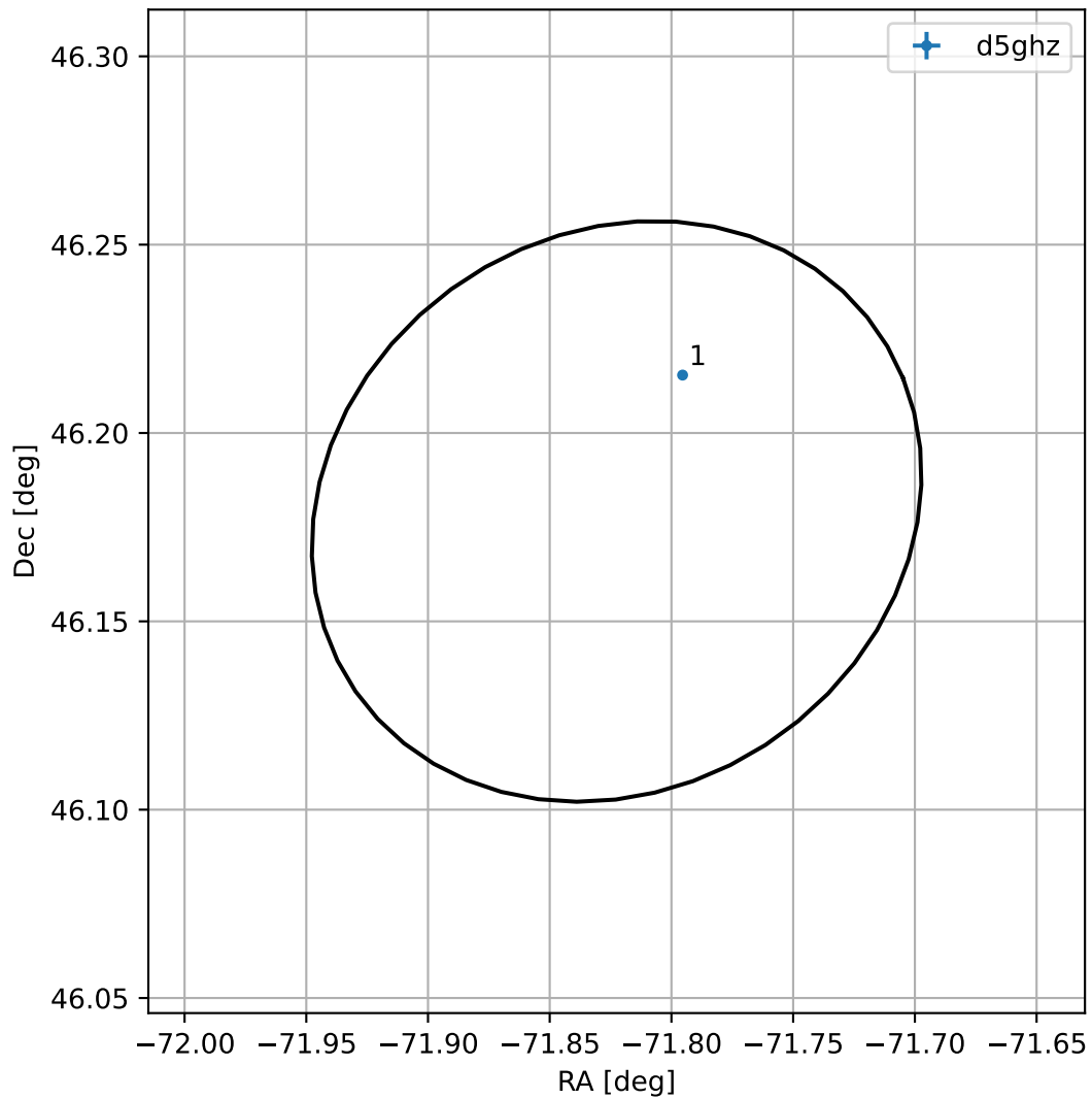
4FGL J1912.7+4610
