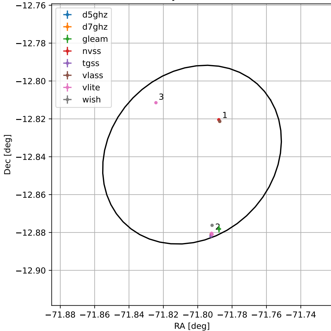
4FGL J1912.7-1250
