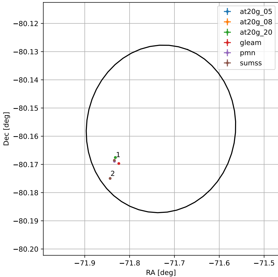
4FGL J1913.0-8009
