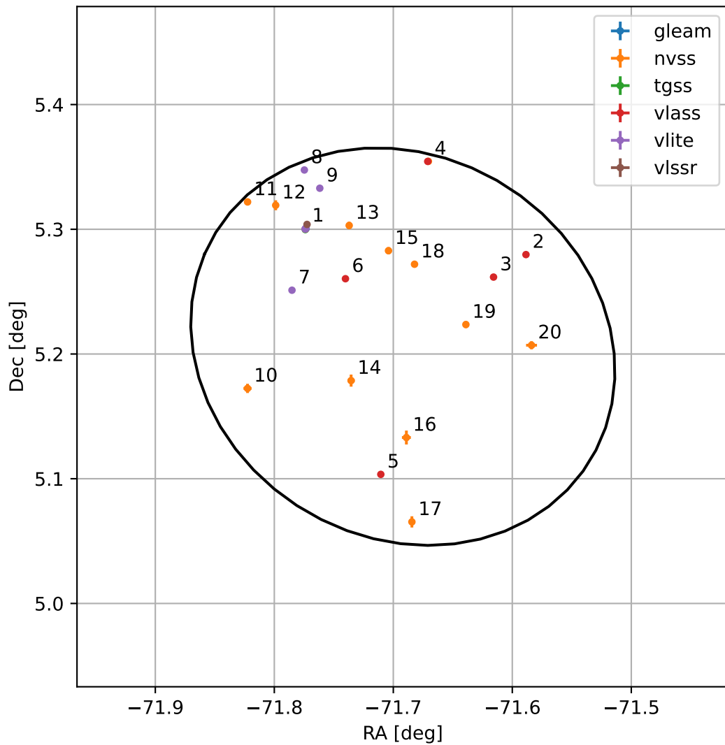
4FGL J1913.2+0512
