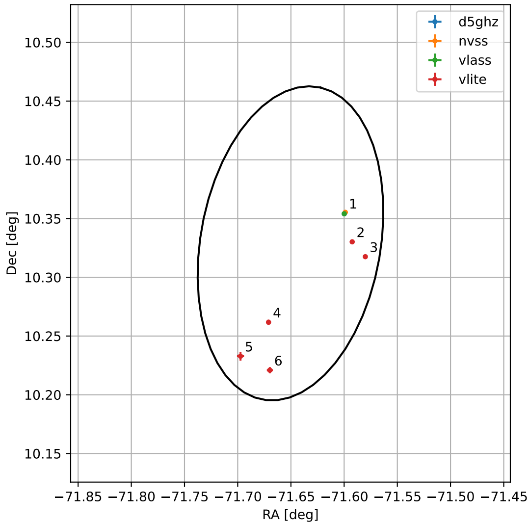
4FGL J1913.3+1019
