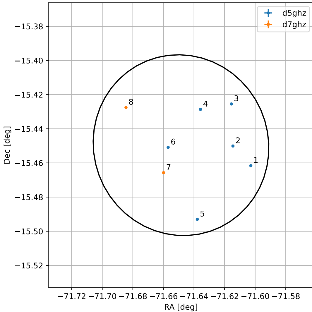
4FGL J1913.4-1526
