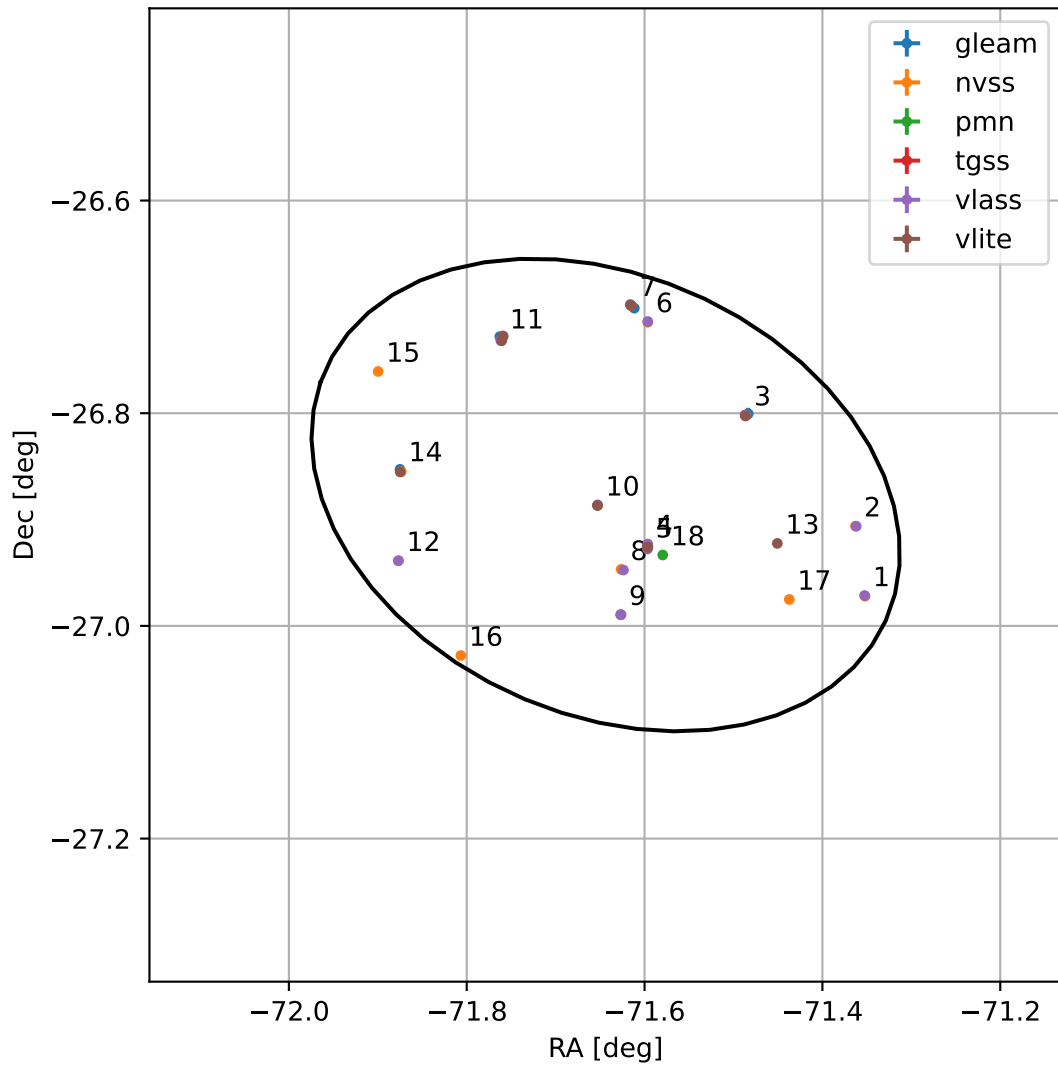
4FGL J1913.4-2652
