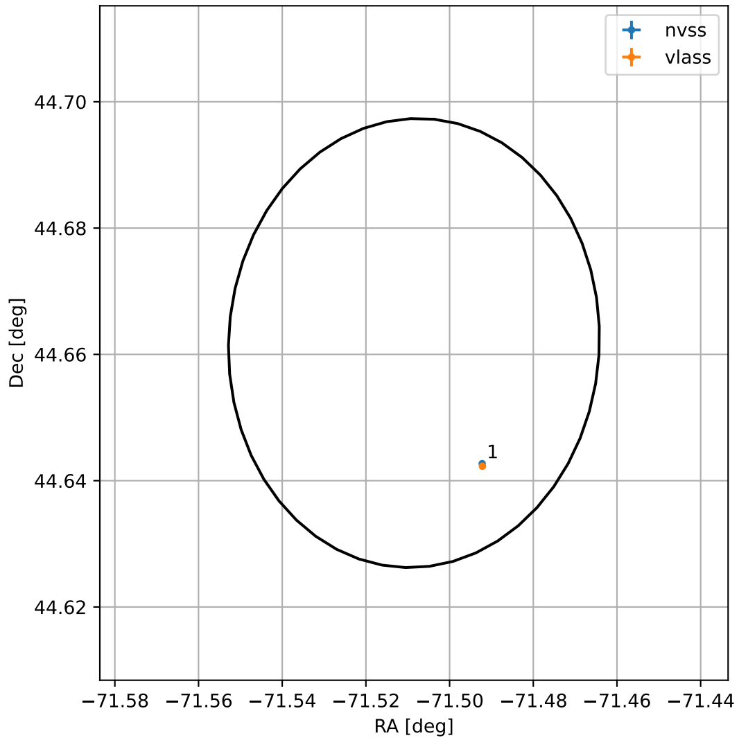
4FGL J1913.9+4439
