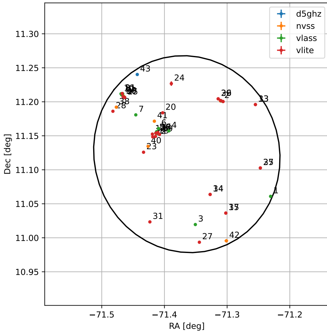
4FGL J1914.5+1107
