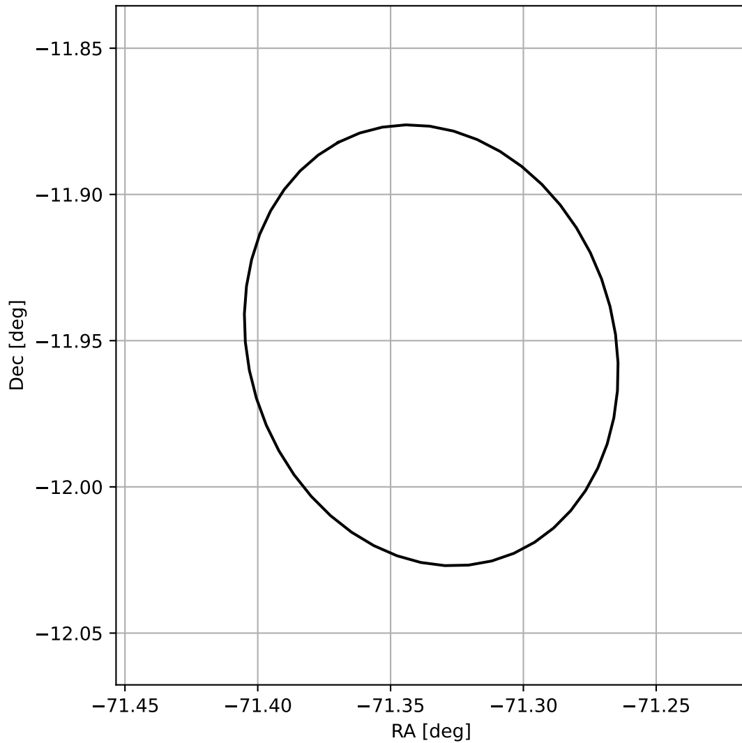
4FGL J1914.6-1157
