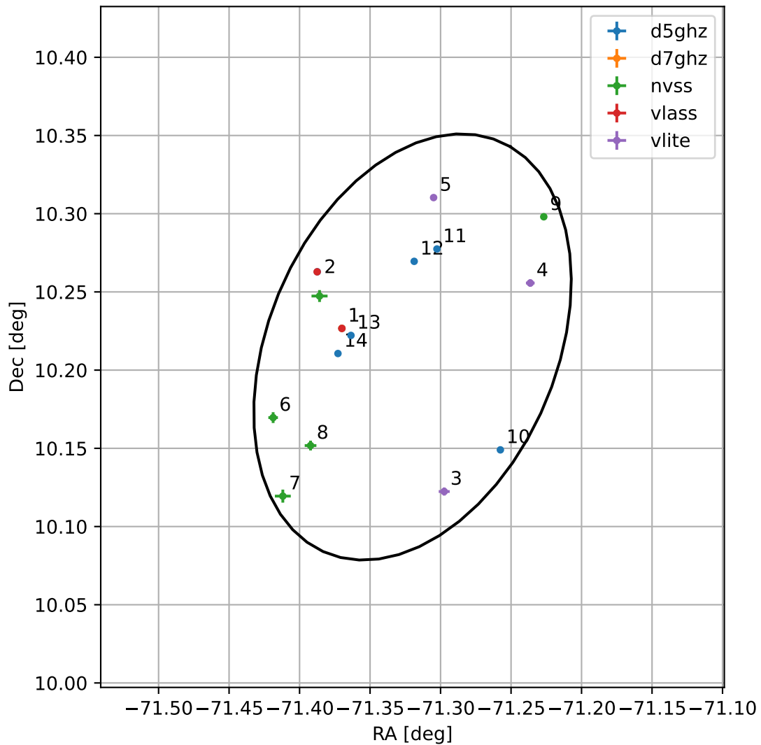
4FGL J1914.7+1012
