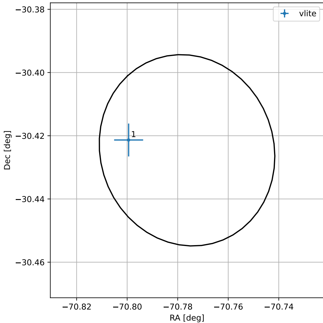
4FGL J1916.8-3025
