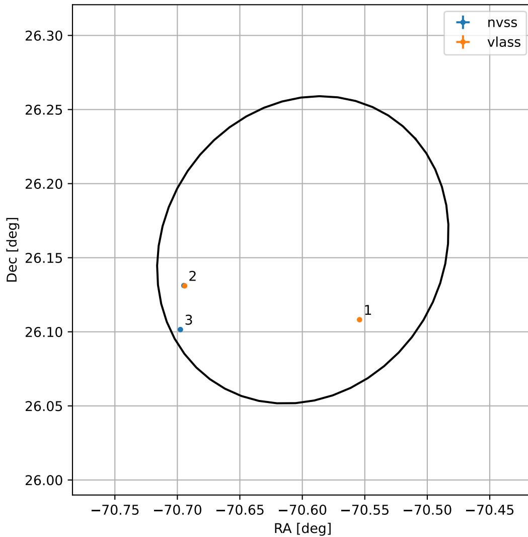
4FGL J1917.6+2609
