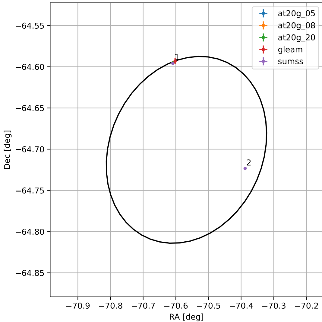
4FGL J1917.7-6442
