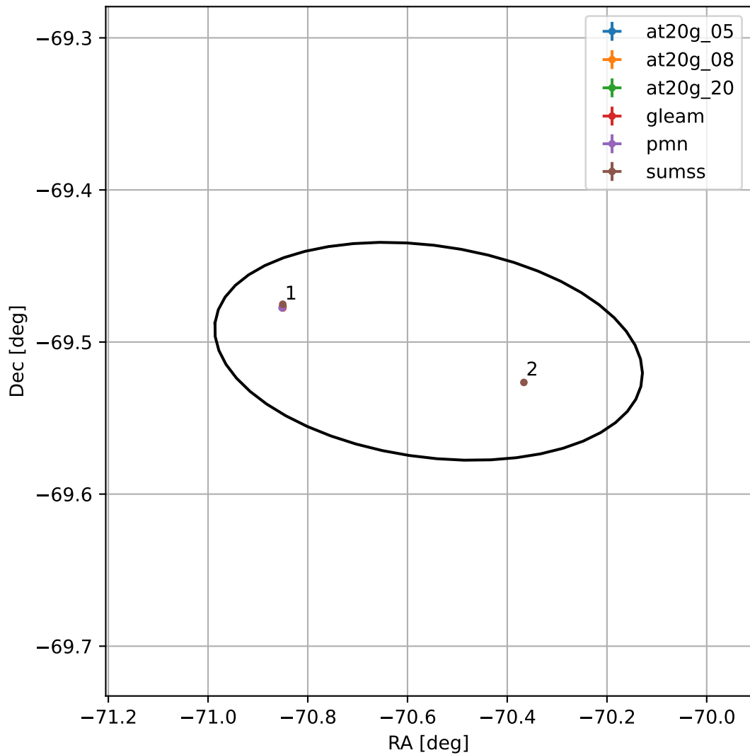
4FGL J1917.7-6930
