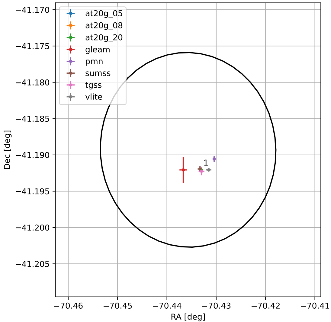
4FGL J1918.2-4111
