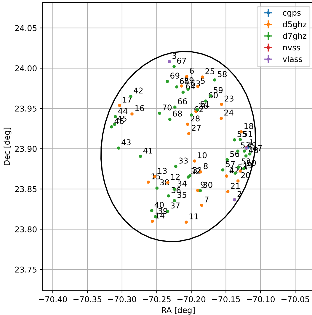
4FGL J1919.1+2354
