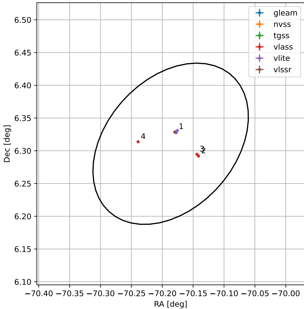
4FGL J1919.2+0618
