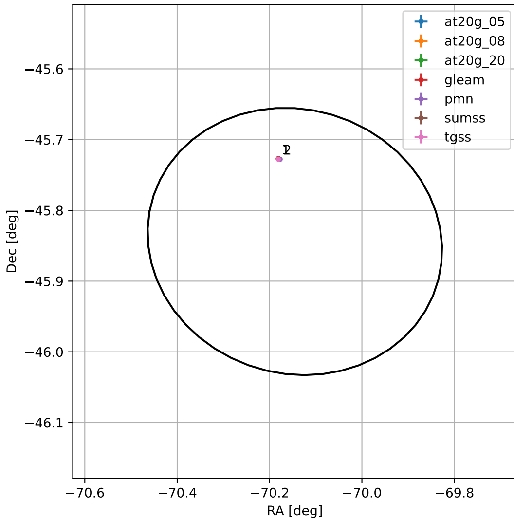
4FGL J1919.4-4550
