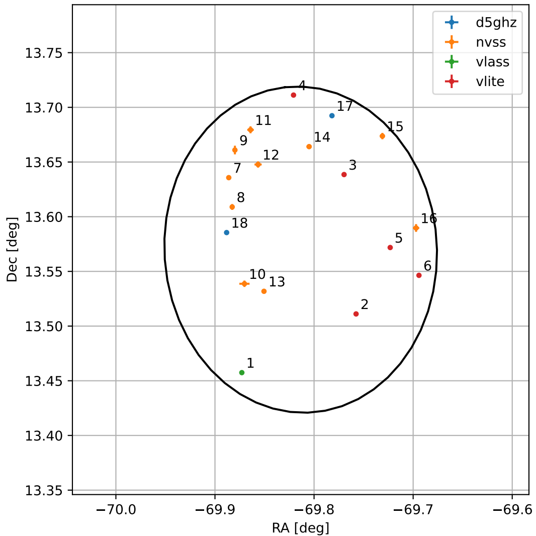
4FGL J1920.7+1334
