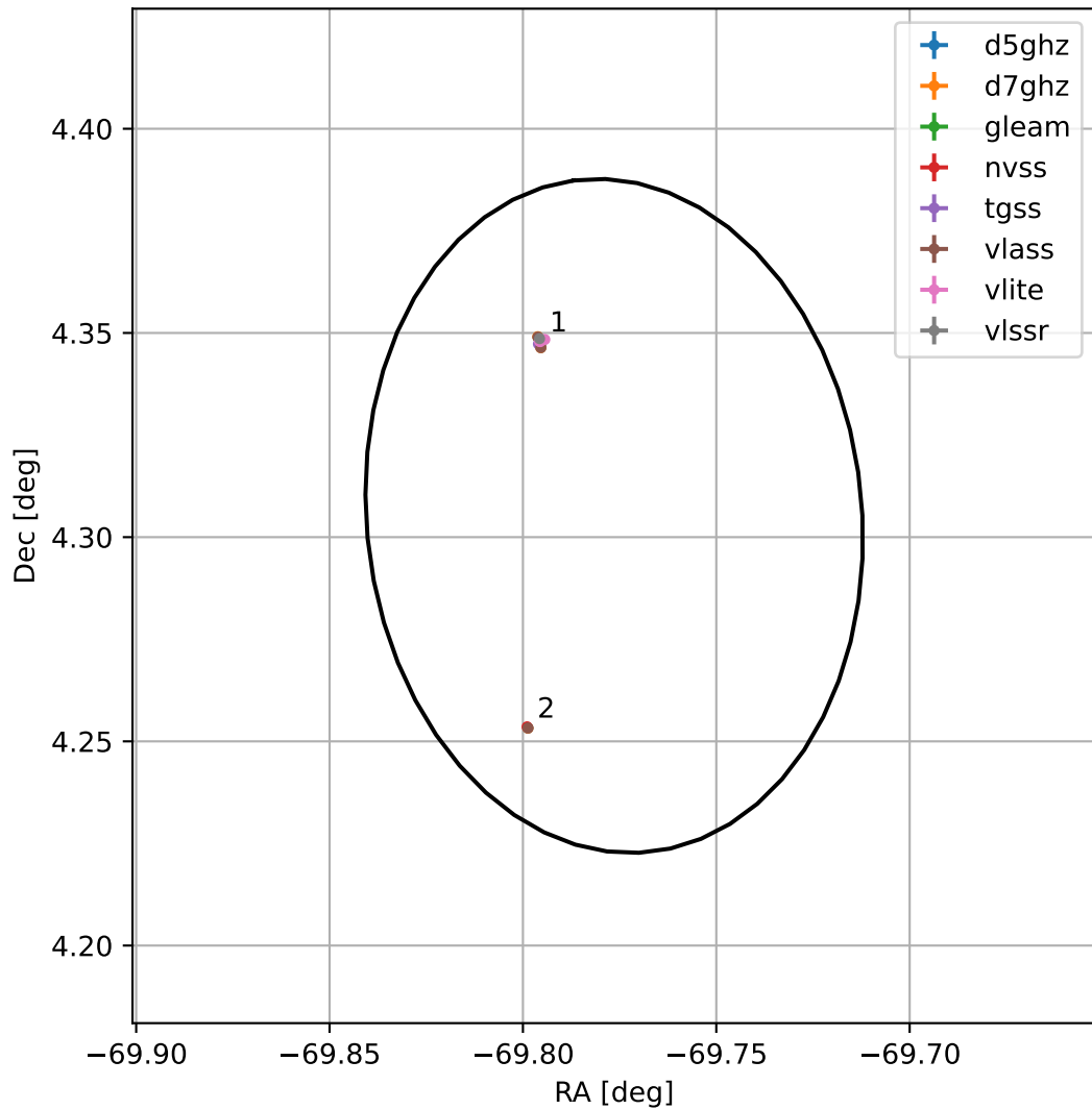
4FGL J1920.8+0418
