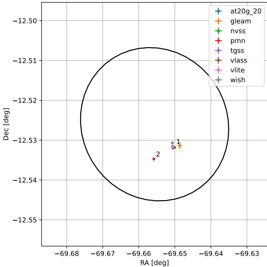
4FGL J1921.3-1231
