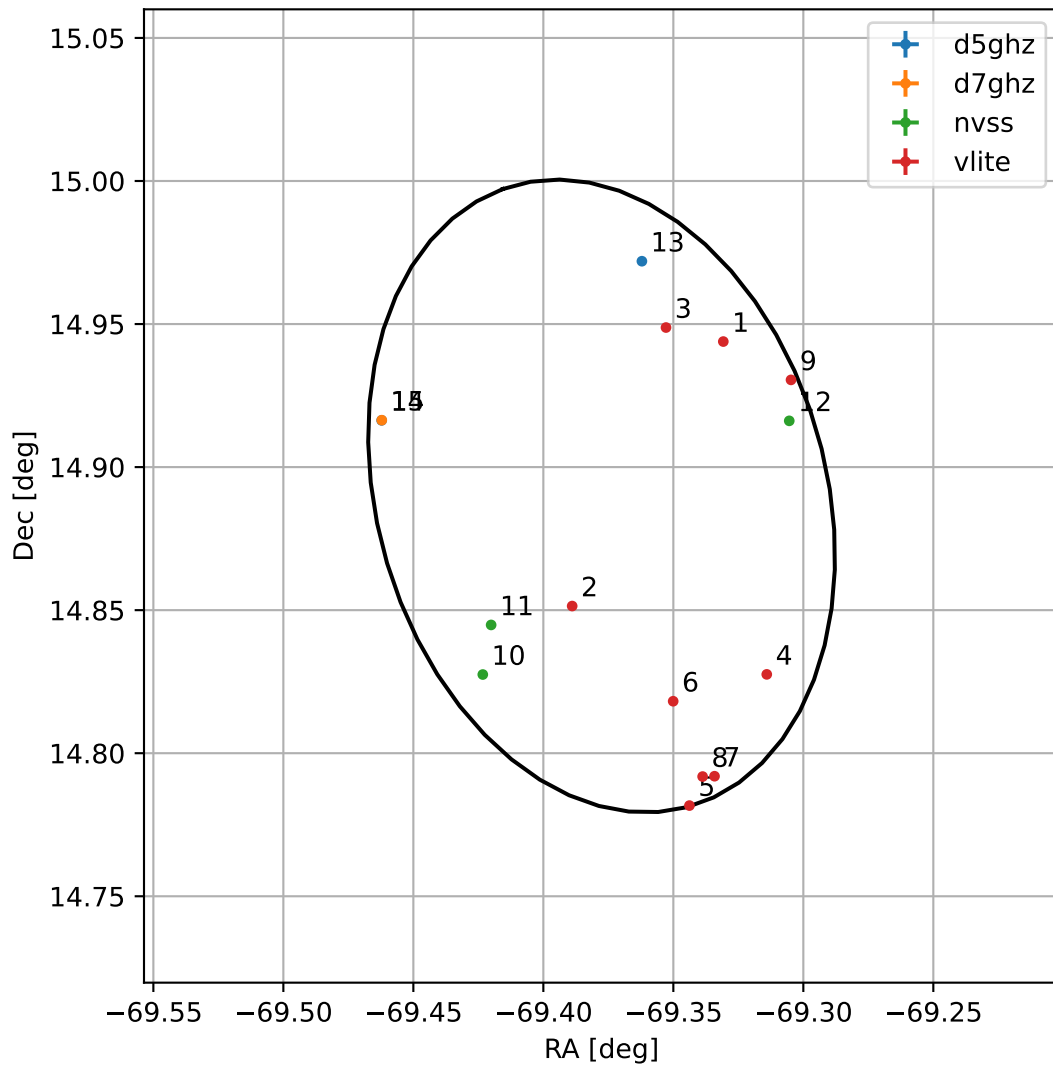
4FGL J1922.4+1453
