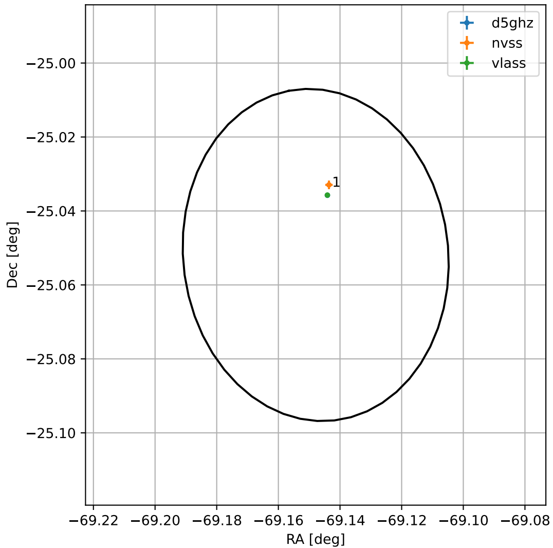
4FGL J1923.4-2503
