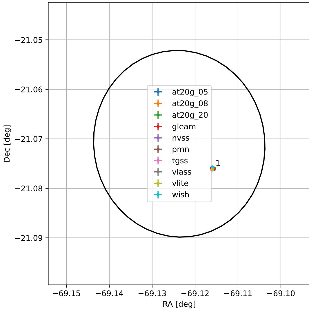
4FGL J1923.5-2104
