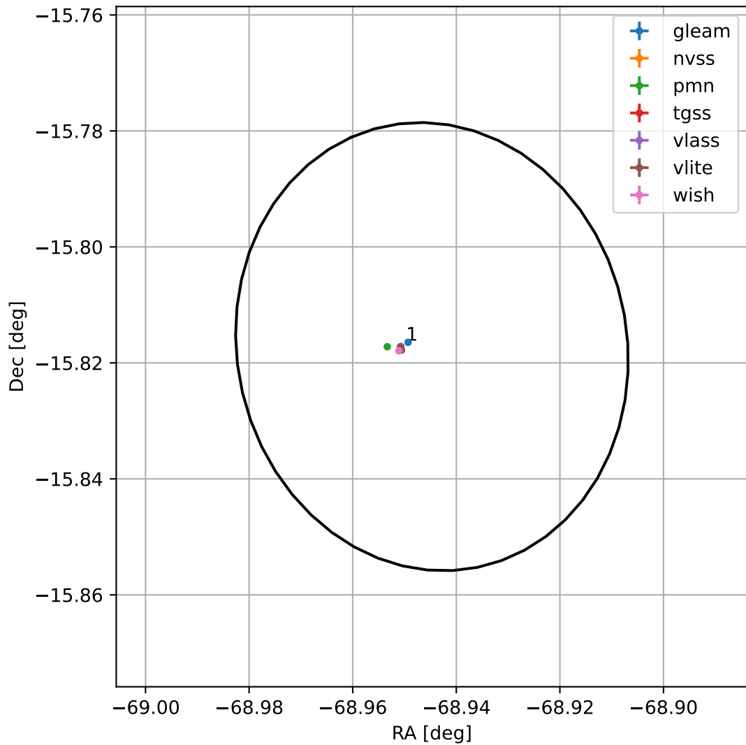
4FGL J1924.2-1549
