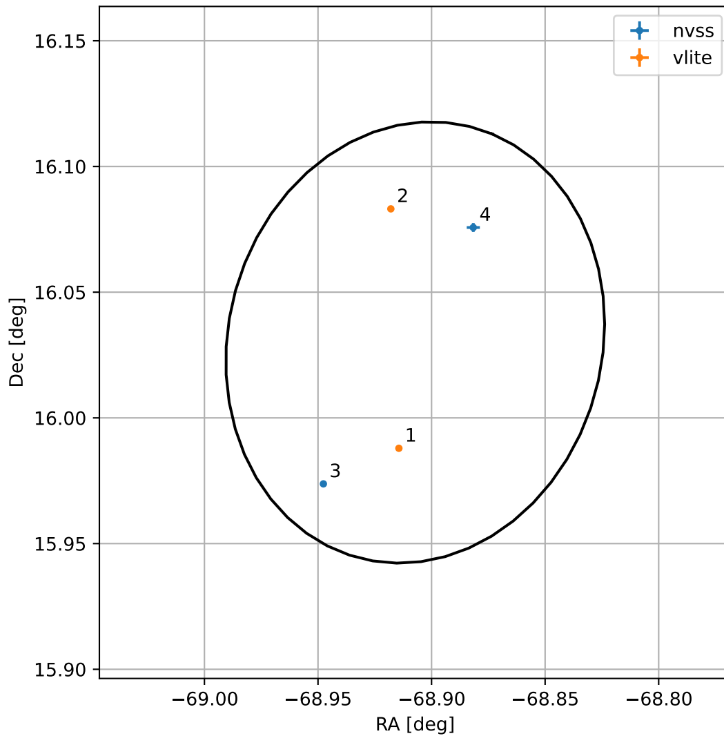
4FGL J1924.3+1601
