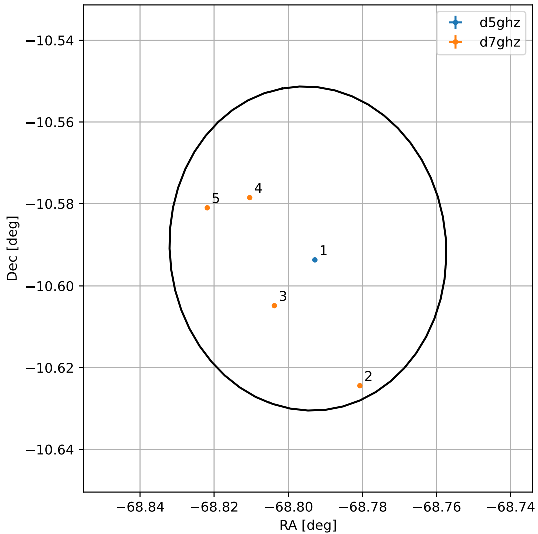
4FGL J1924.8-1035
