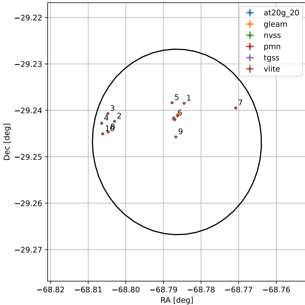
4FGL J1924.8-2914
