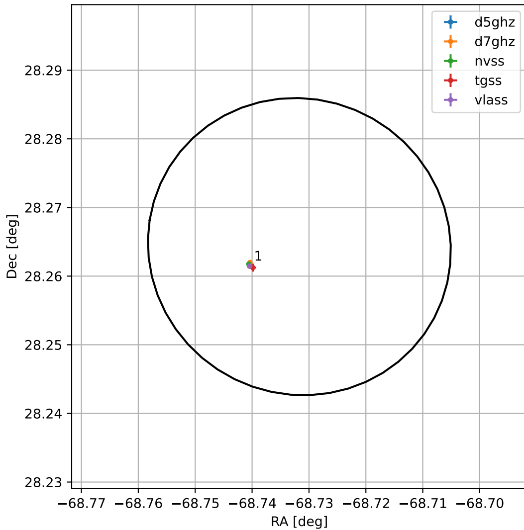
4FGL J1925.0+2815
