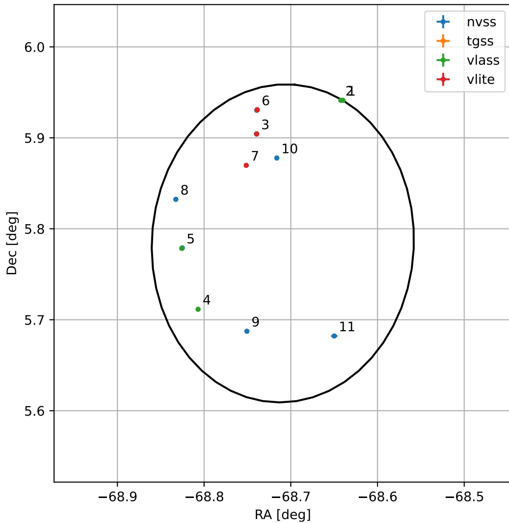
4FGL J1925.1+0547
