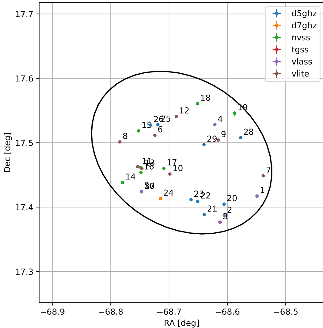
4FGL J1925.2+1729
