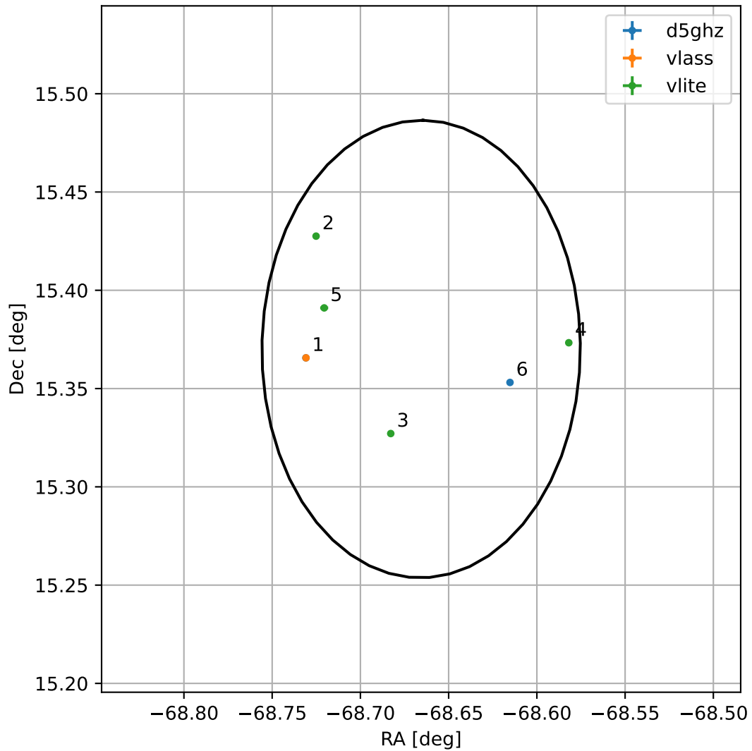
4FGL J1925.3+1522
