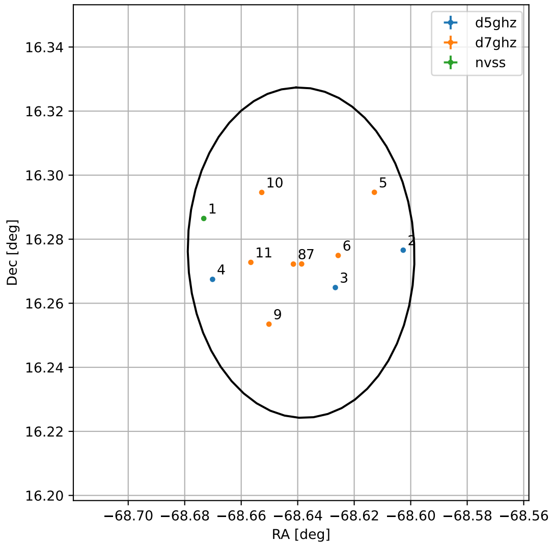
4FGL J1925.4+1616
