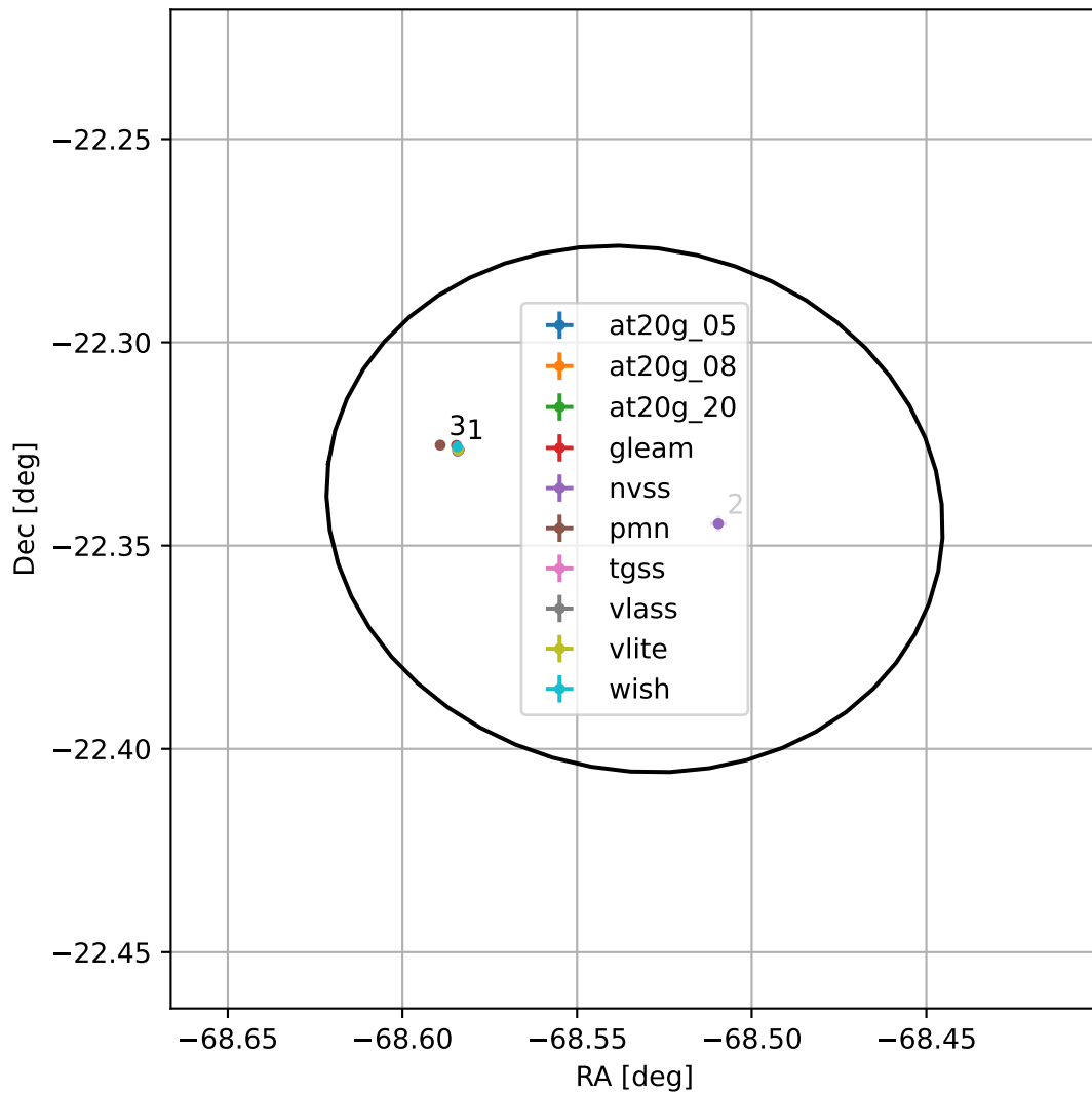
4FGL J1925.8-2220
