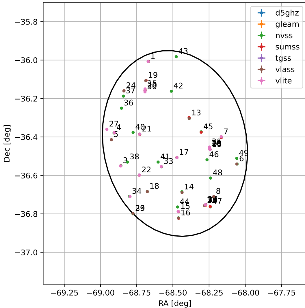
4FGL J1926.0-3626
