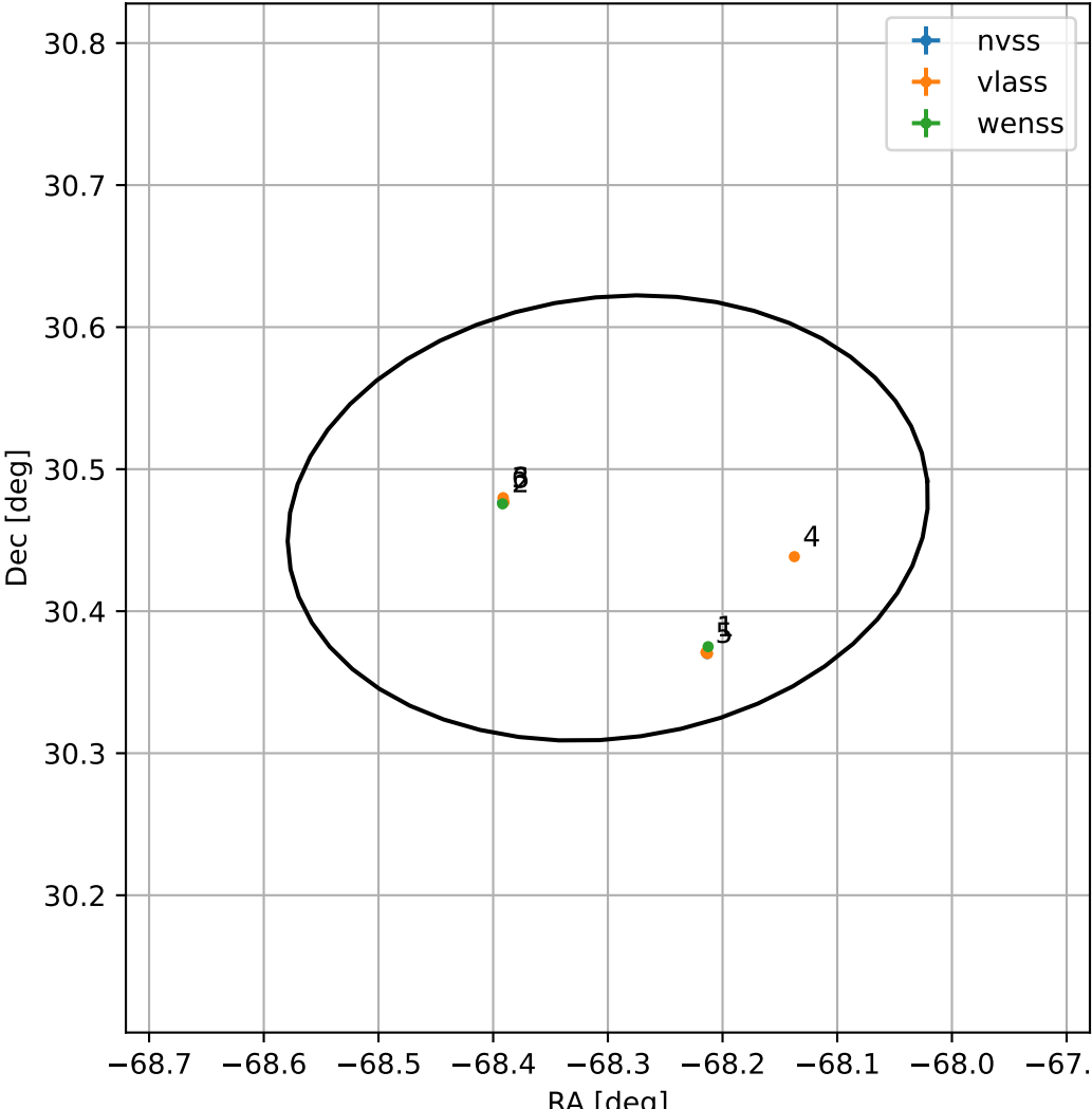
4FGL J1926.7+3027
