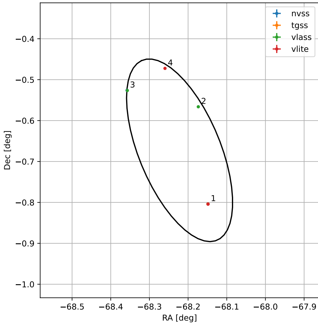
4FGL J1927.1-0040
