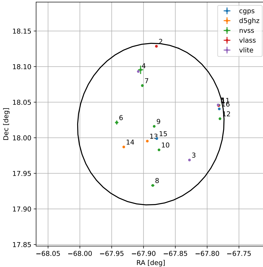
4FGL J1928.4+1801
