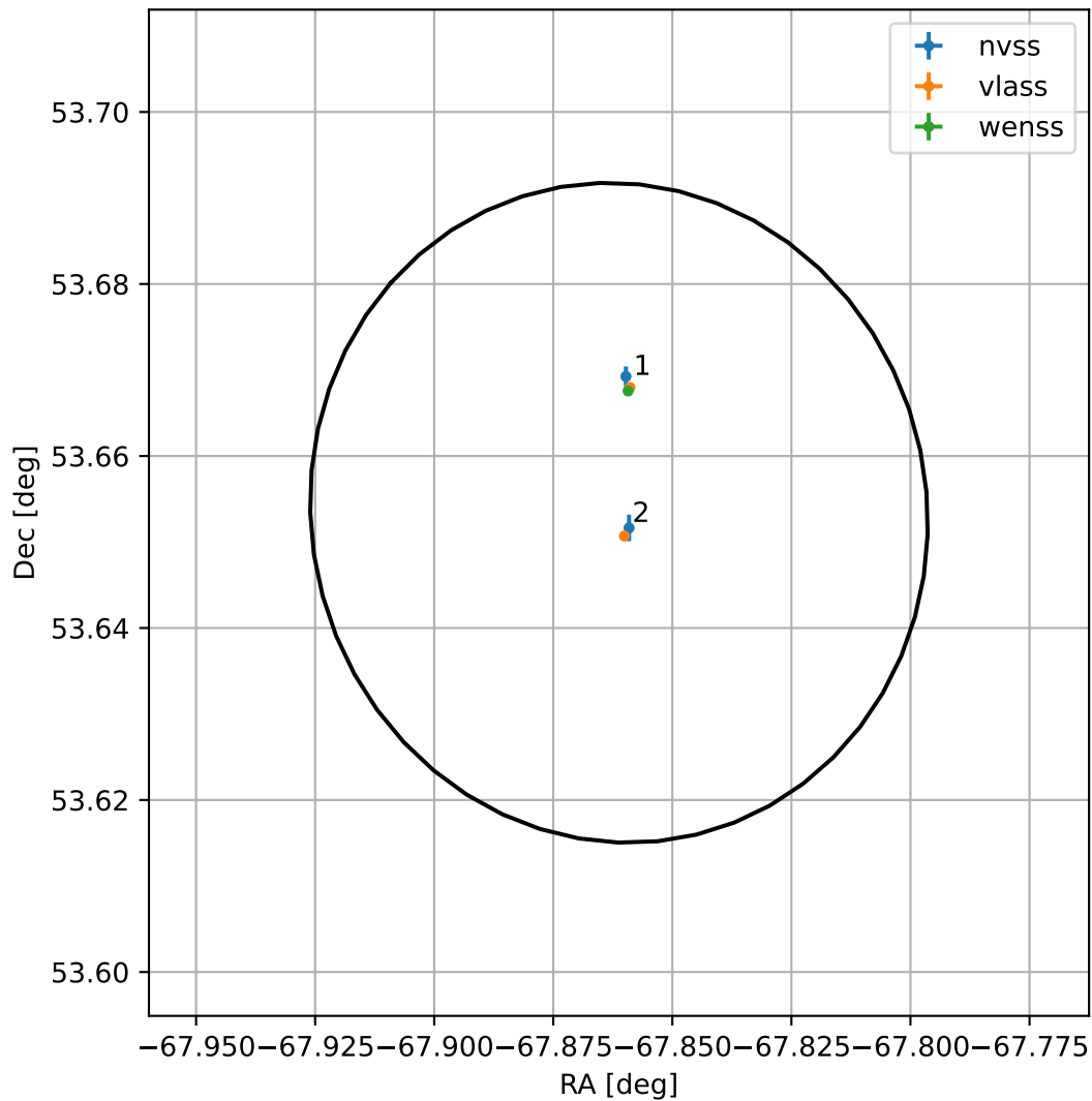
4FGL J1928.5+5339
