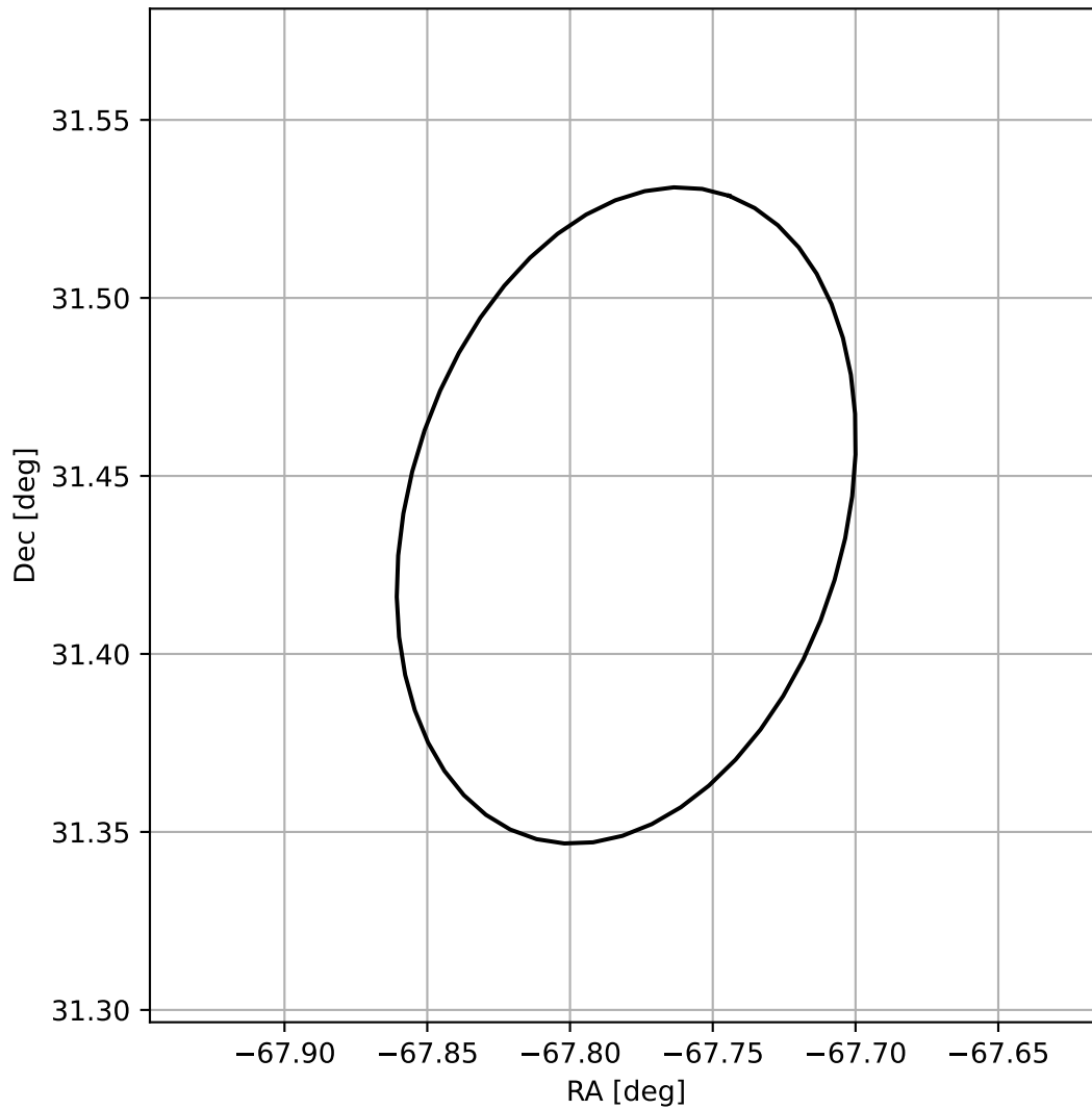
4FGL J1928.8+3126
