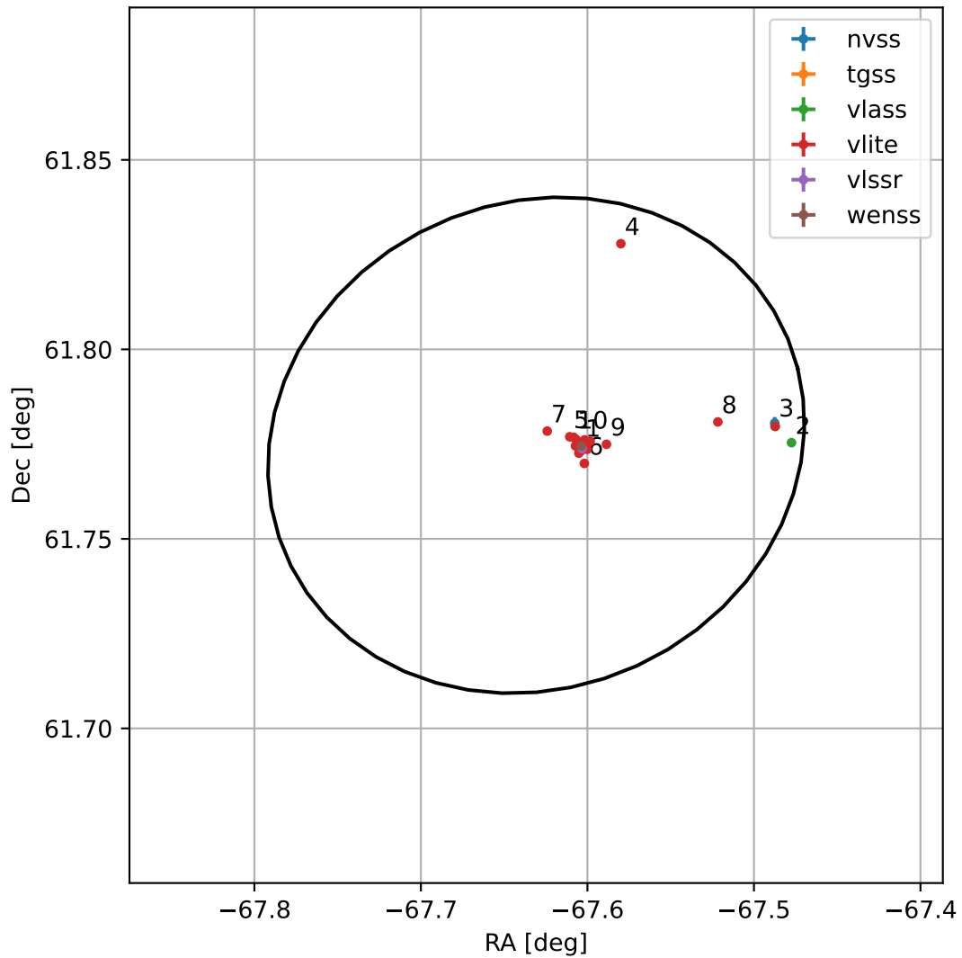
4FGL J1929.4+6146
