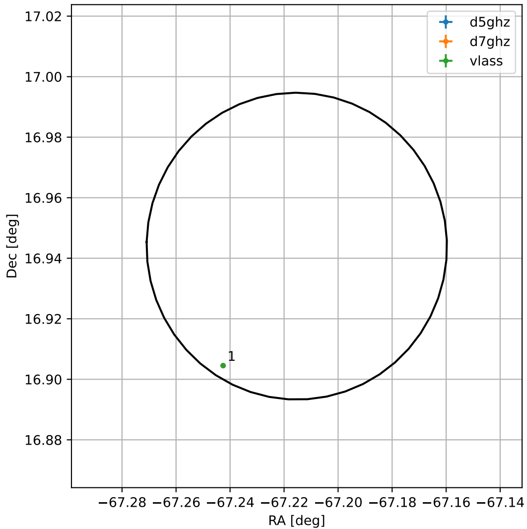
4FGL J1931.1+1656
